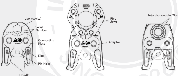
Standard Pressing Jaws
